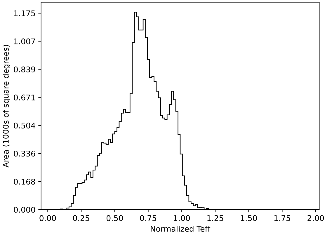
noroll_mjdp120_v3.4_10yrs All sky all bands: Normalized Teff
