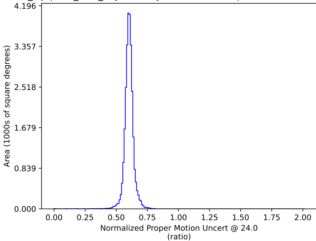
noroll_mjdp120_v3.4_10yrs All sky: Normalized Proper Motion Uncert @ 24.0
