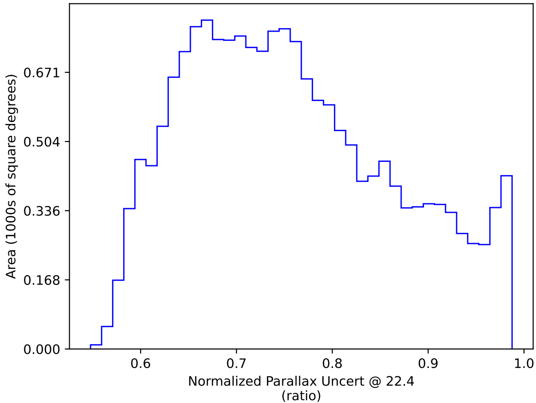
noroll_mjdp120_v3.4_10yrs WFD: Normalized Parallax Uncert @ 22.4
