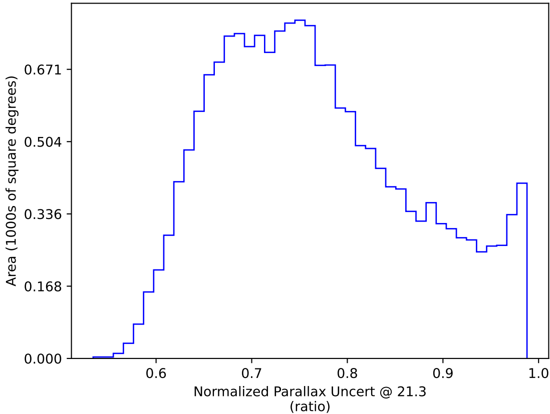
noroll_mjdp120_v3.4_10yrs WFD y band only: Normalized Parallax Uncert @ 21.3
