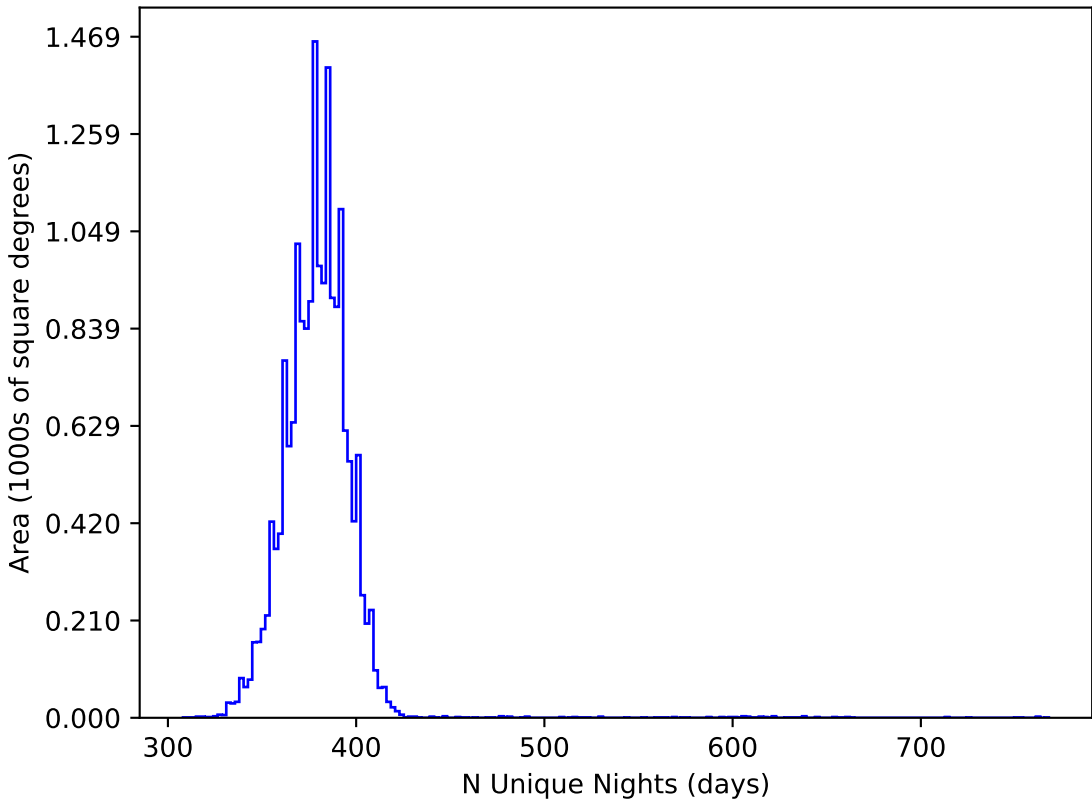
noroll_mjdp120_v3.4_10yrs WFD all bands: N Unique Nights
