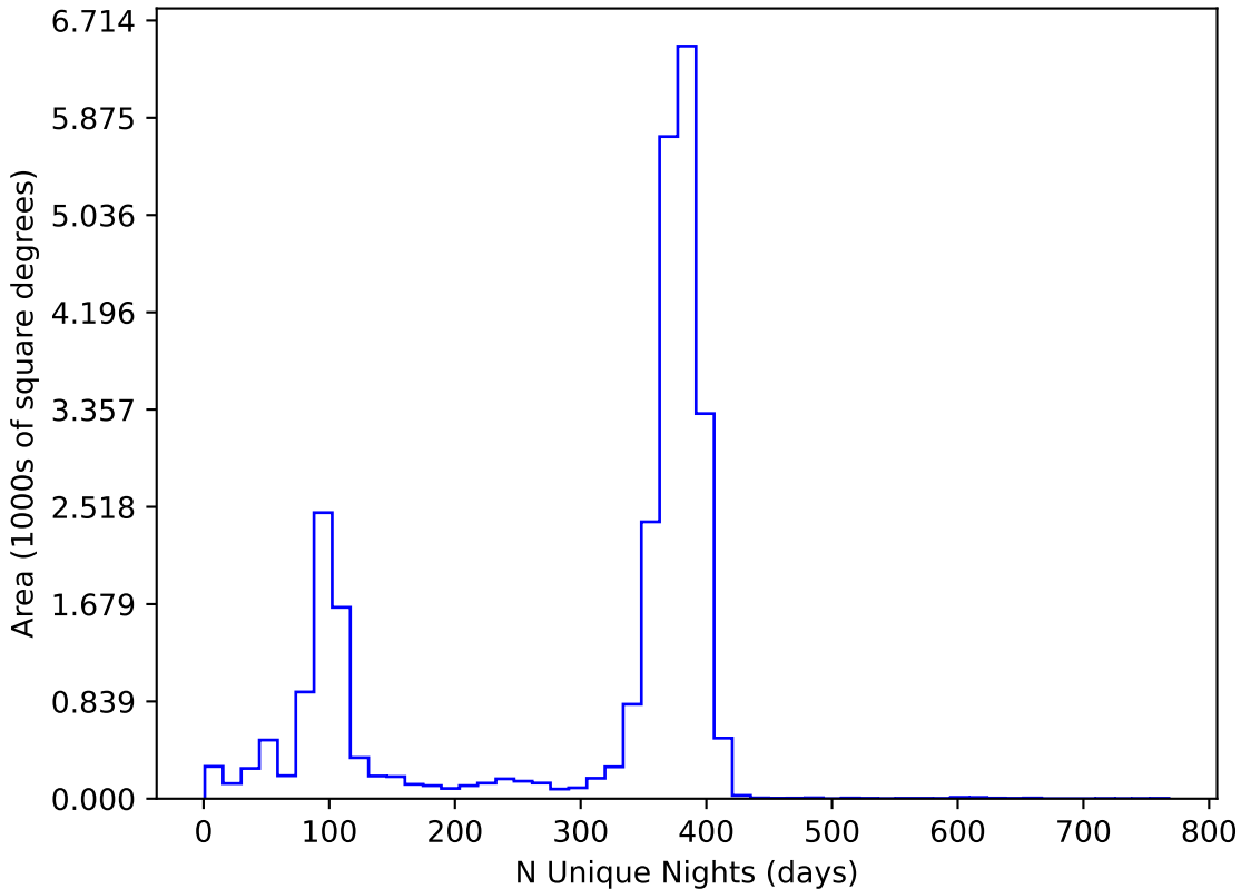
noroll_mjdp120_v3.4_10yrs All sky all bands: N Unique Nights
