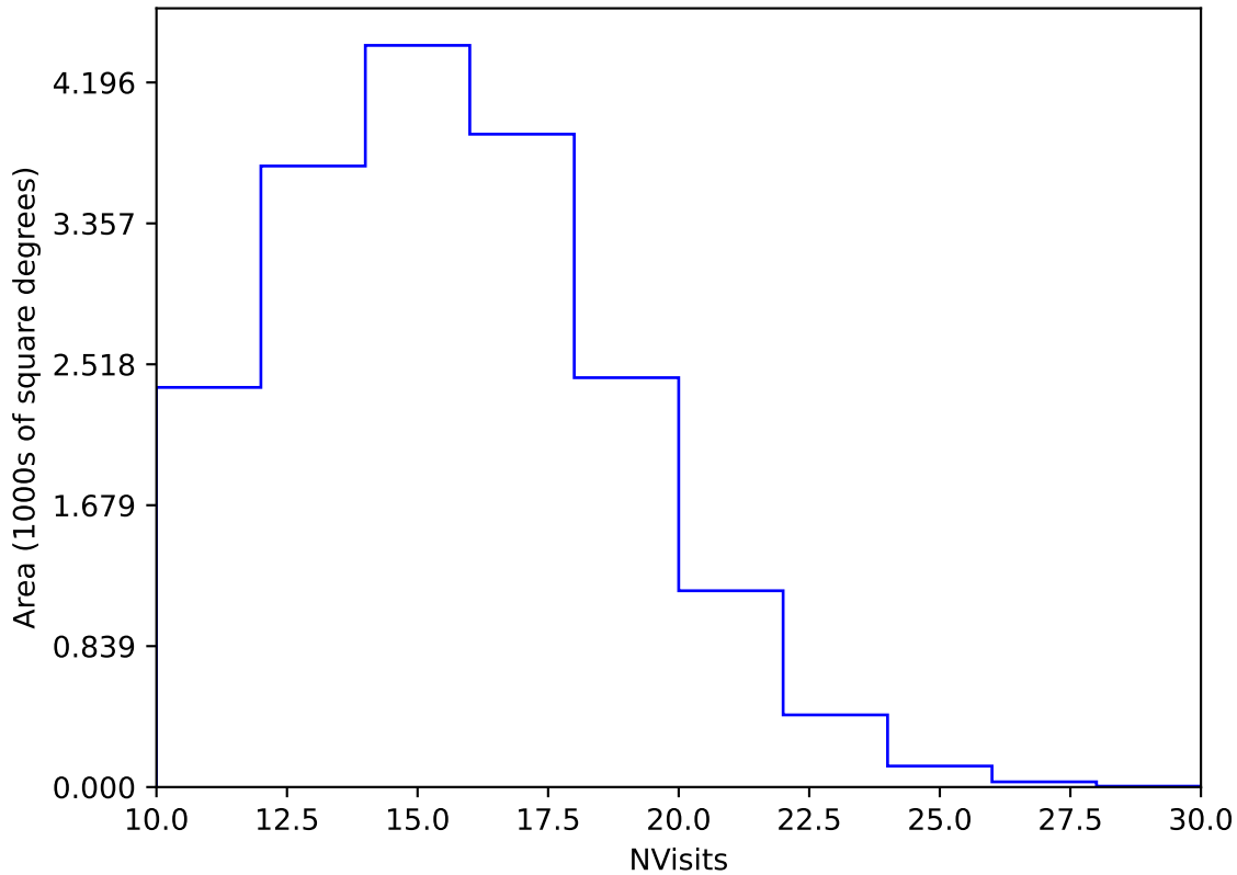
noroll_mjdp120_v3.4_10yrs Yr 3-4 y band: NVisits
