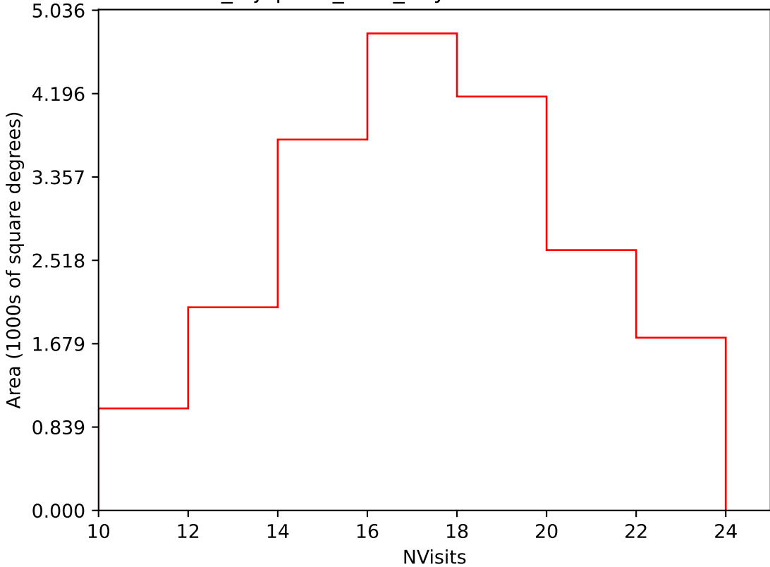
noroll_mjdp120_v3.4_10yrs Yr 3-4 i band: NVisits
