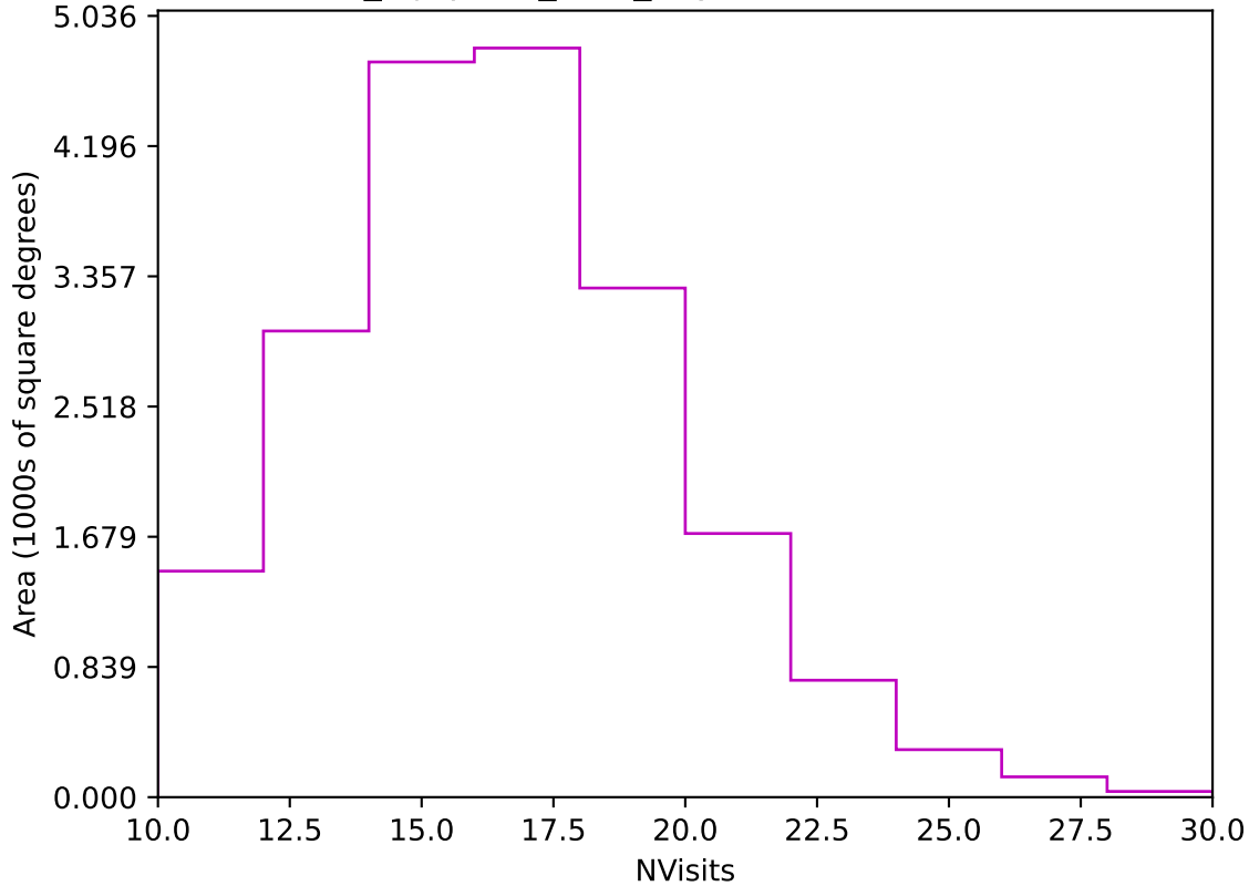
noroll_mjdp120_v3.4_10yrs Yr 1 z band: NVisits
