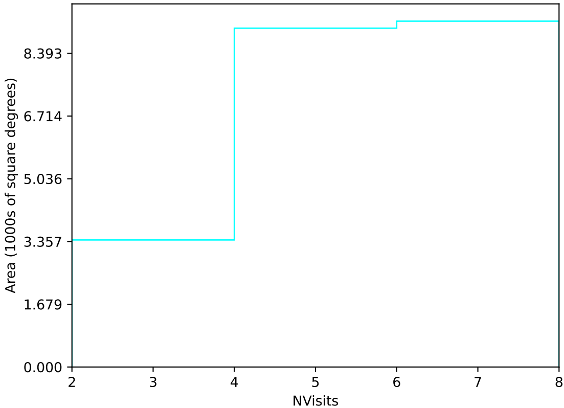
noroll_mjdp120_v3.4_10yrs Yr 1 u band: NVisits
