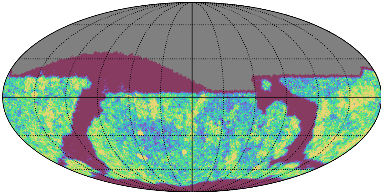
noroll_mjdp120_v3.4_10yrs Yr 1 i band: NVisits
