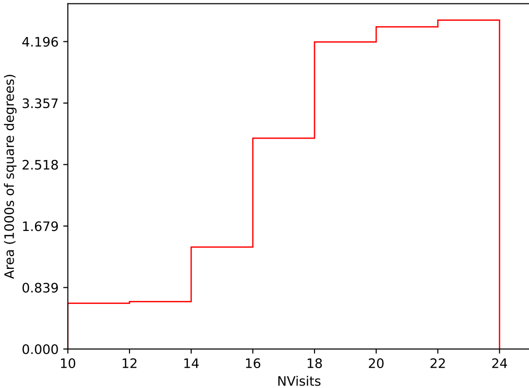
noroll_mjdp120_v3.4_10yrs Yr 1 i band: NVisits
