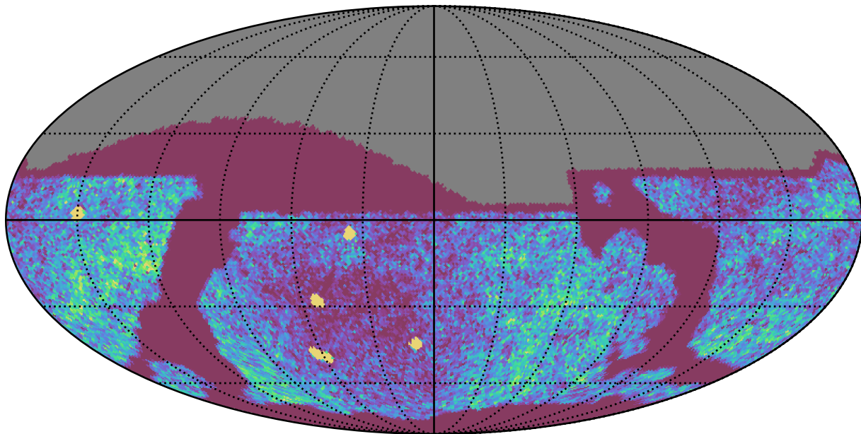
noroll_mjdp120_v3.4_10yrs Yr 1 all bands: NVisits
