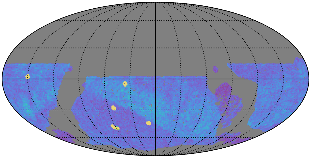
noroll_mjdp120_v3.4_10yrs WFD z band: NVisits
