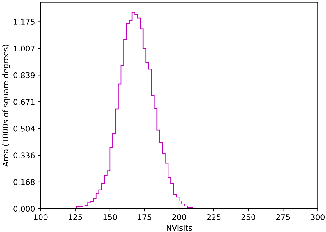
noroll_mjdp120_v3.4_10yrs WFD z band: NVisits
