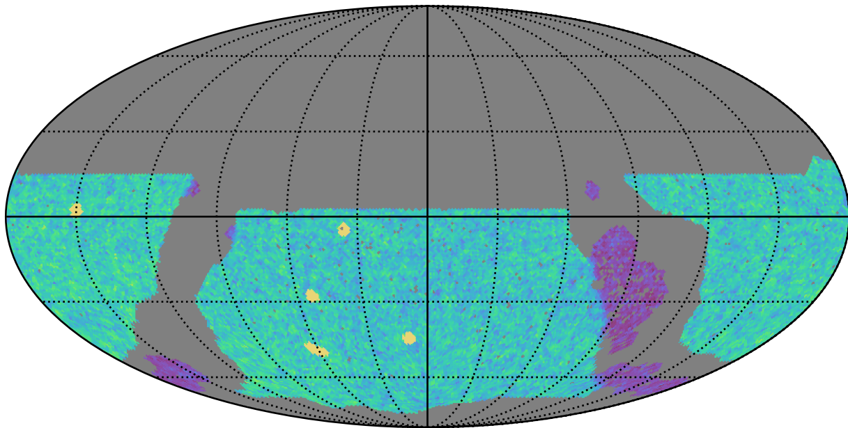
noroll_mjdp120_v3.4_10yrs WFD u band: NVisits
