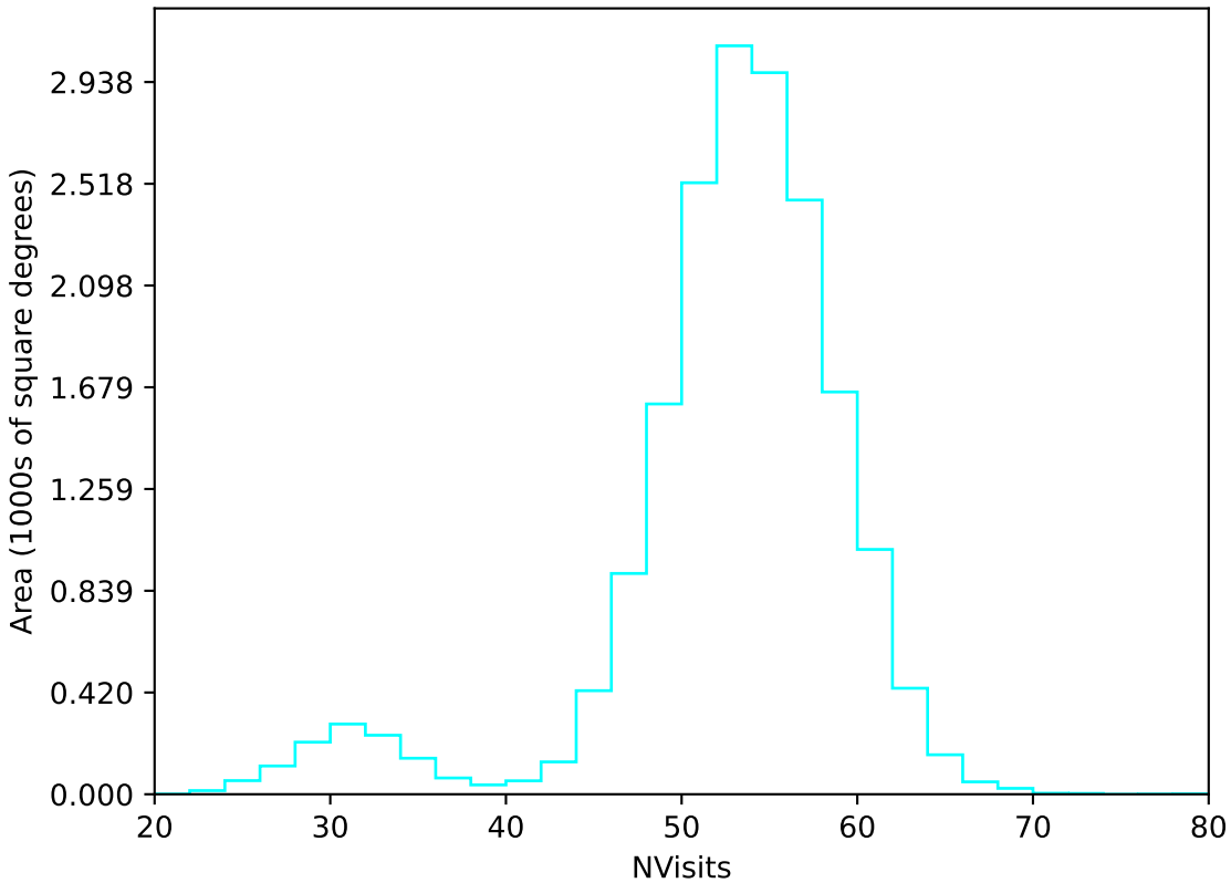
noroll_mjdp120_v3.4_10yrs WFD u band: NVisits
