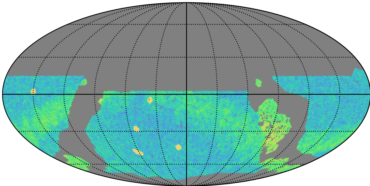
noroll_mjdp120_v3.4_10yrs WFD r band: NVisits
