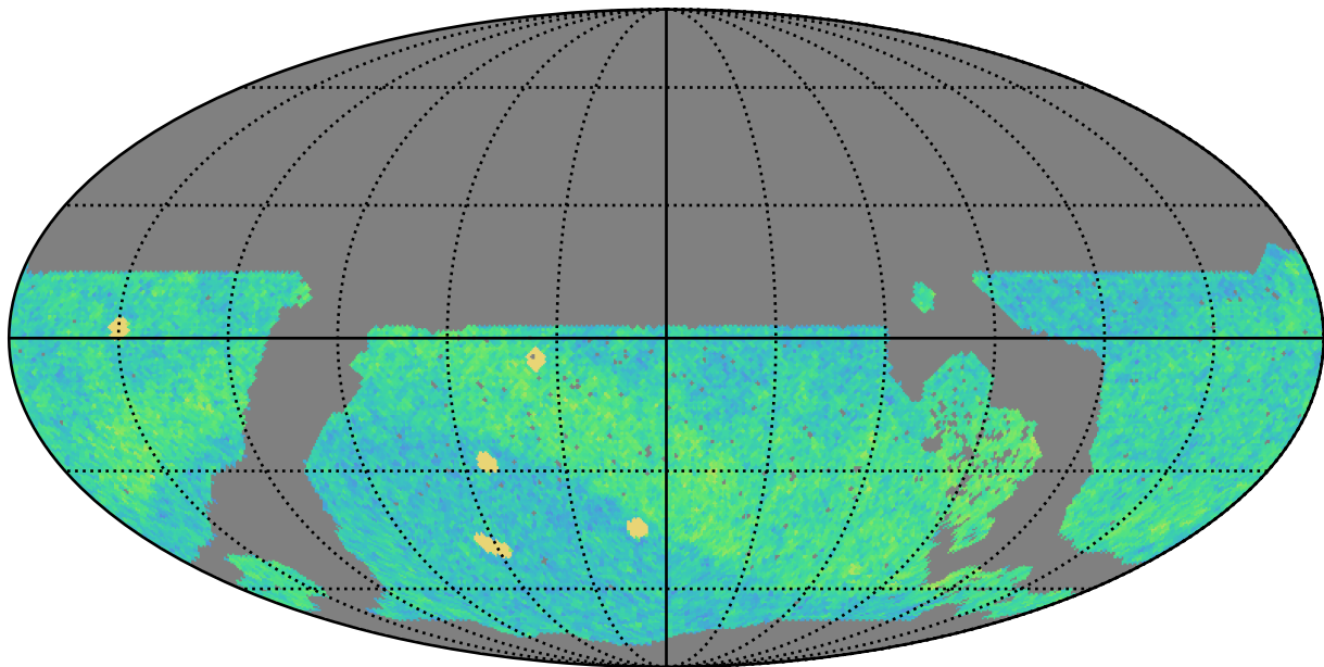
noroll_mjdp120_v3.4_10yrs WFD i band: NVisits
