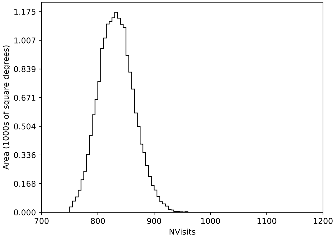
noroll_mjdp120_v3.4_10yrs WFD all bands: NVisits
