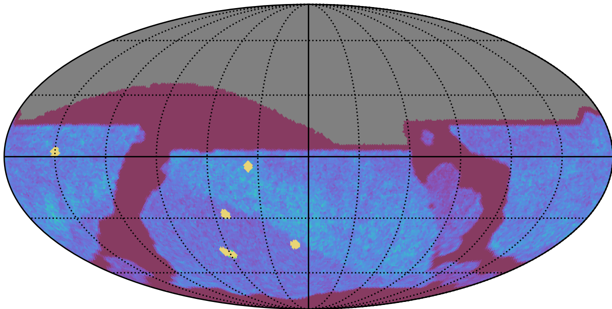
noroll_mjdp120_v3.4_10yrs All sky z band: NVisits
