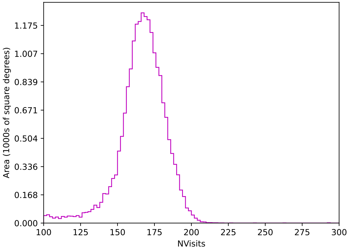
noroll_mjdp120_v3.4_10yrs All sky z band: NVisits
