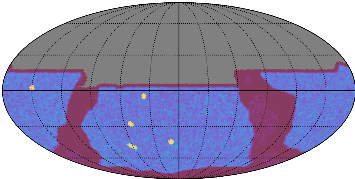
noroll_mjdp120_v3.4_10yrs All sky y band: NVisits
