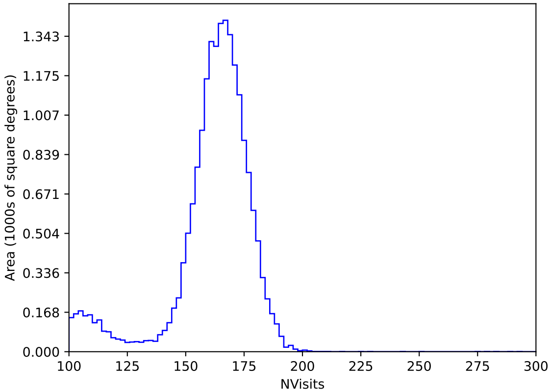
noroll_mjdp120_v3.4_10yrs All sky y band: NVisits
