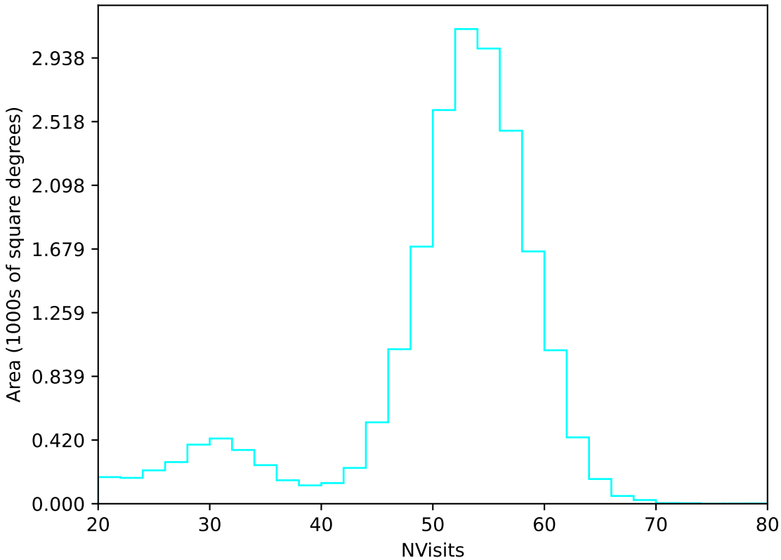
noroll_mjdp120_v3.4_10yrs All sky u band: NVisits
