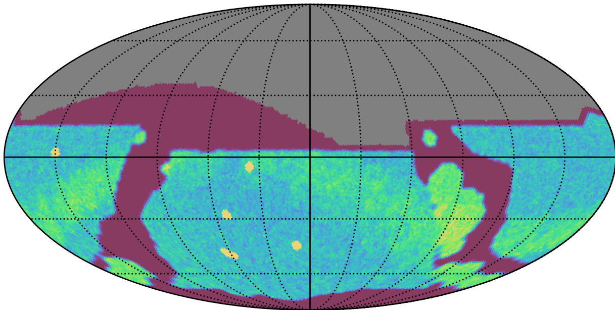
noroll_mjdp120_v3.4_10yrs All sky r band: NVisits
