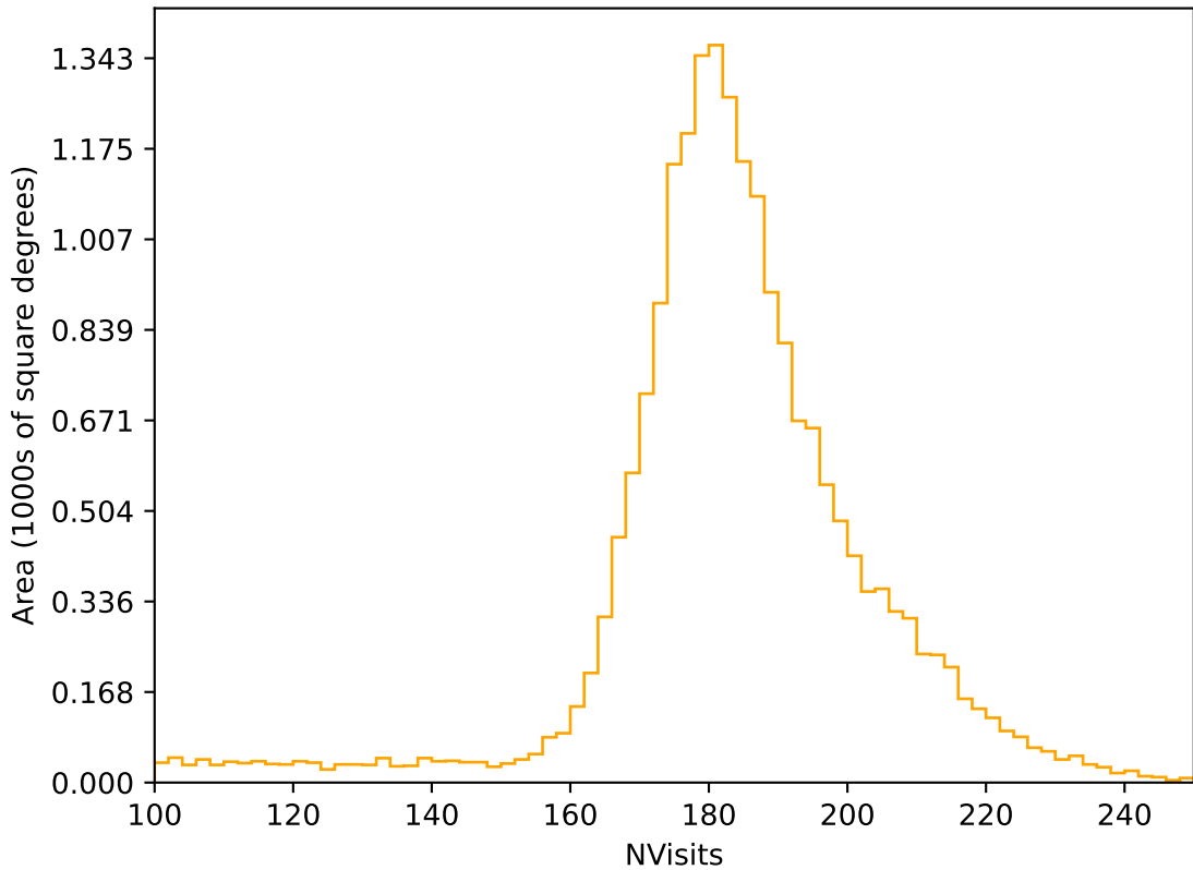
noroll_mjdp120_v3.4_10yrs All sky r band: NVisits
