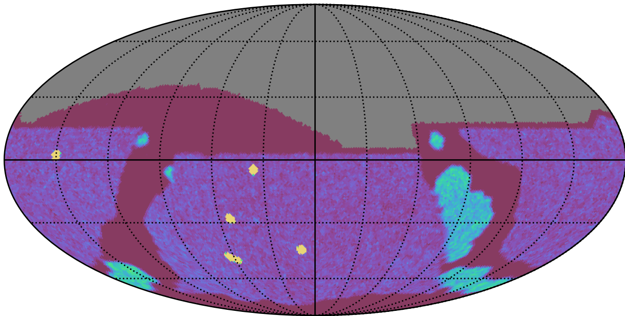
noroll_mjdp120_v3.4_10yrs All sky g band: NVisits
