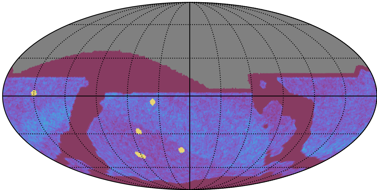
noroll_mjdp120_v3.4_10yrs All sky all bands: NVisits
