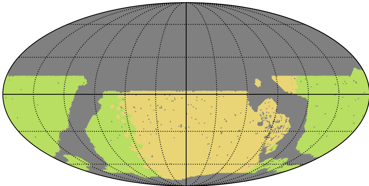
noroll_mjdp120_v3.4_10yrs WFD all bands: NSeasons
