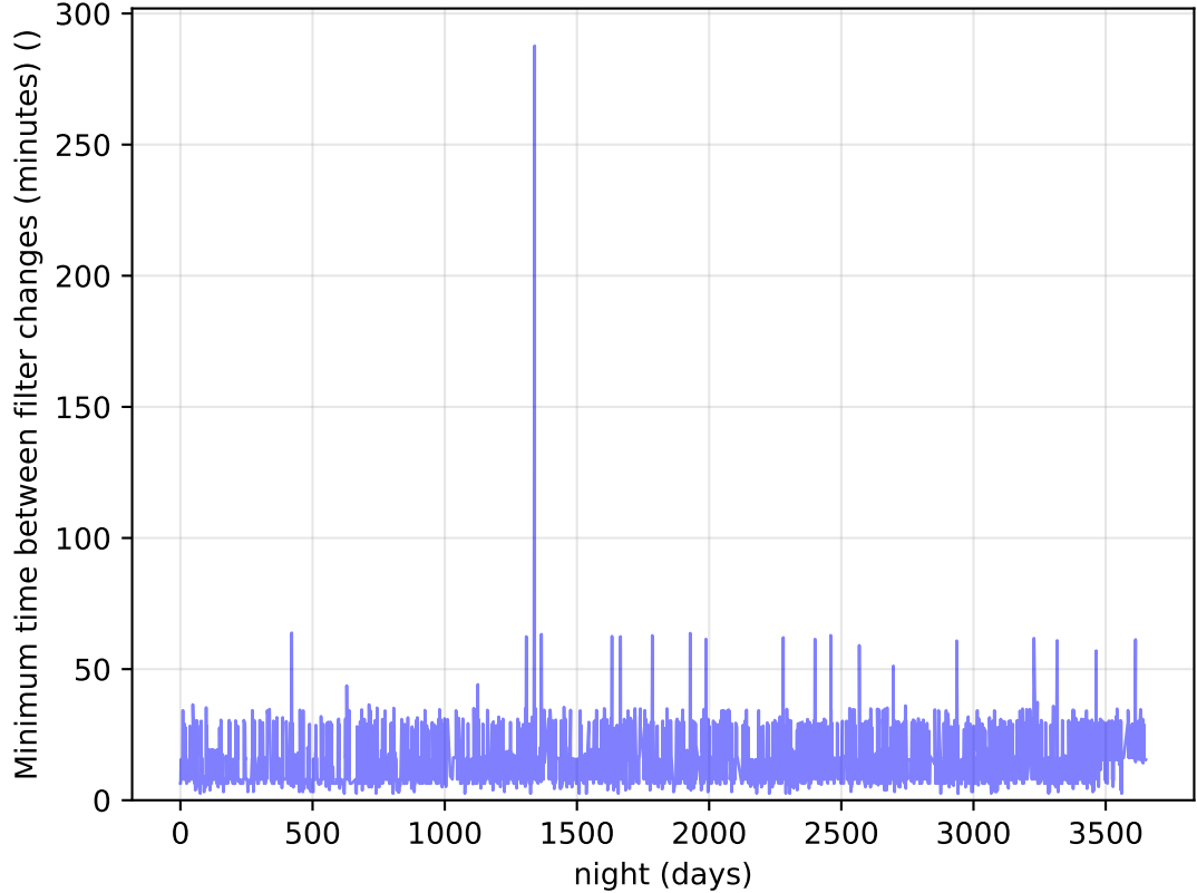
noroll_mjdp120_v3.4_10yrs Per Night: Minimum time between filter changes (minutes)
