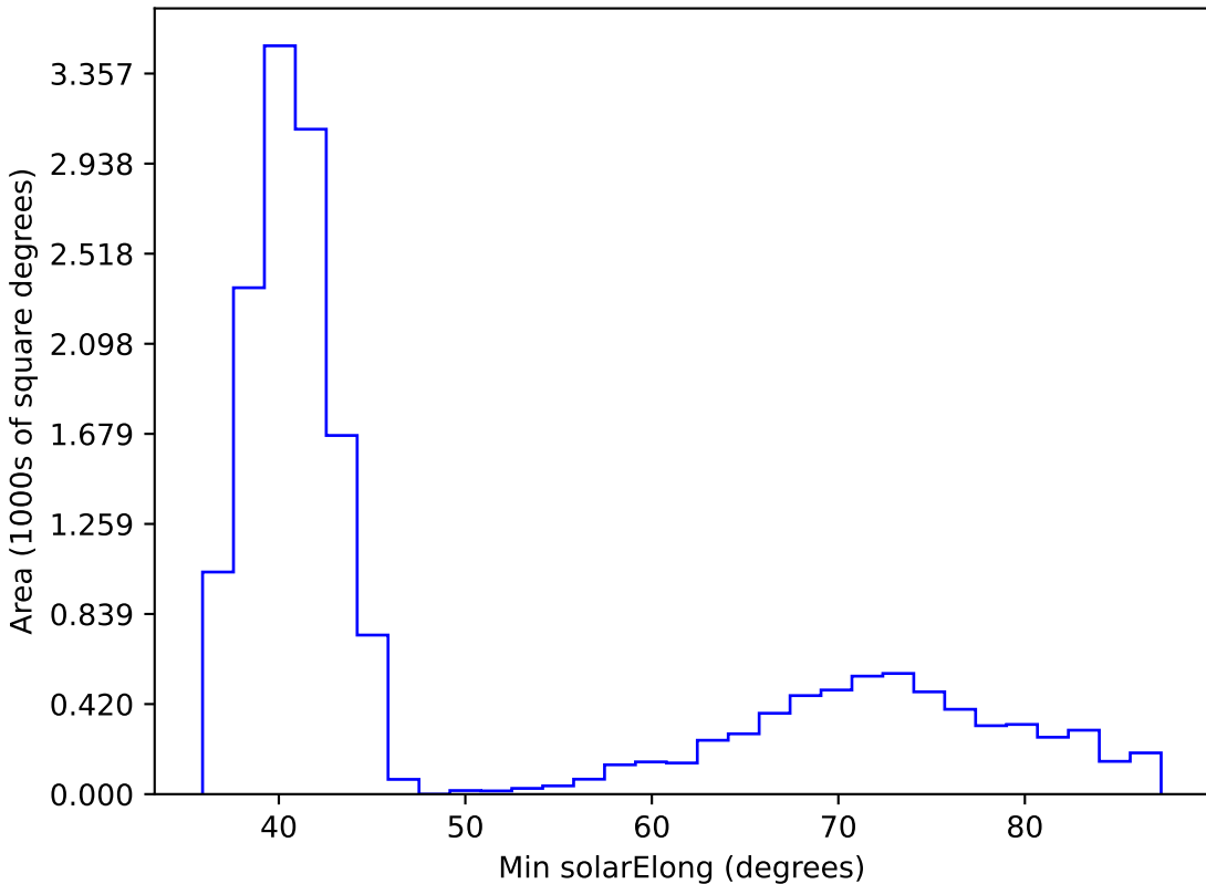
noroll_mjdp120_v3.4_10yrs WFD z band: Min solarElong
