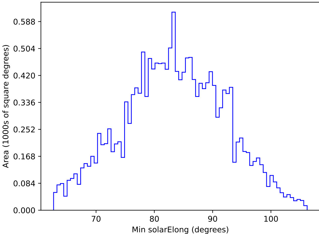
noroll_mjdp120_v3.4_10yrs WFD u band: Min solarElong
