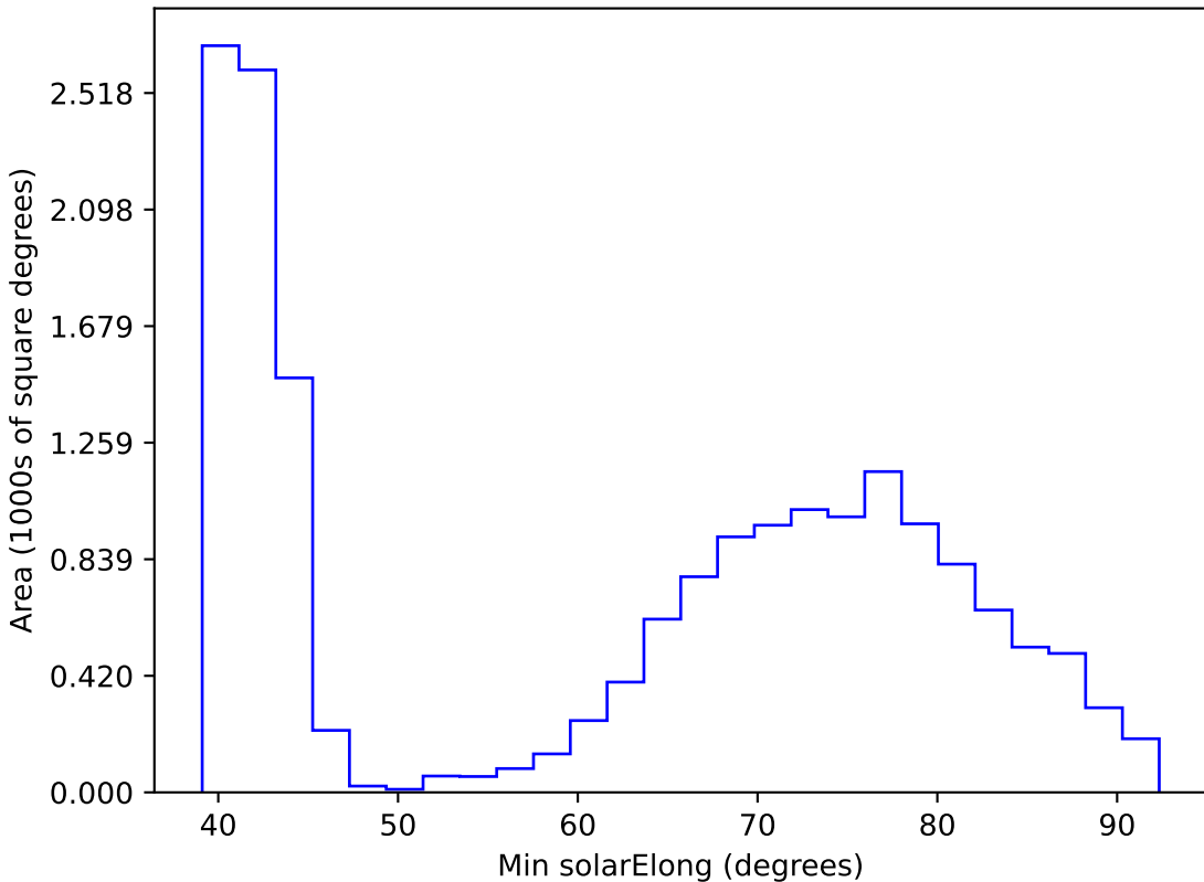
noroll_mjdp120_v3.4_10yrs WFD r band: Min solarElong
