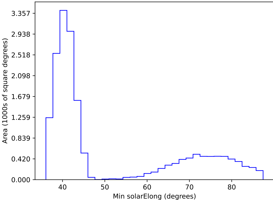
noroll_mjdp120_v3.4_10yrs WFD i band: Min solarElong
