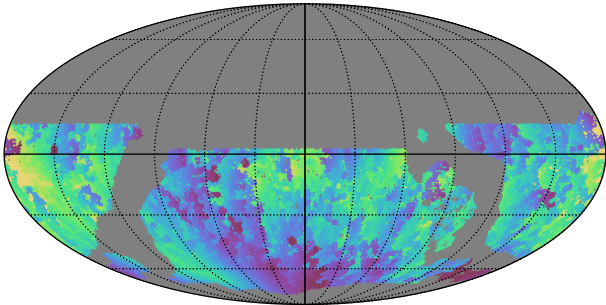
noroll_mjdp120_v3.4_10yrs WFD g band: Min solarElong
