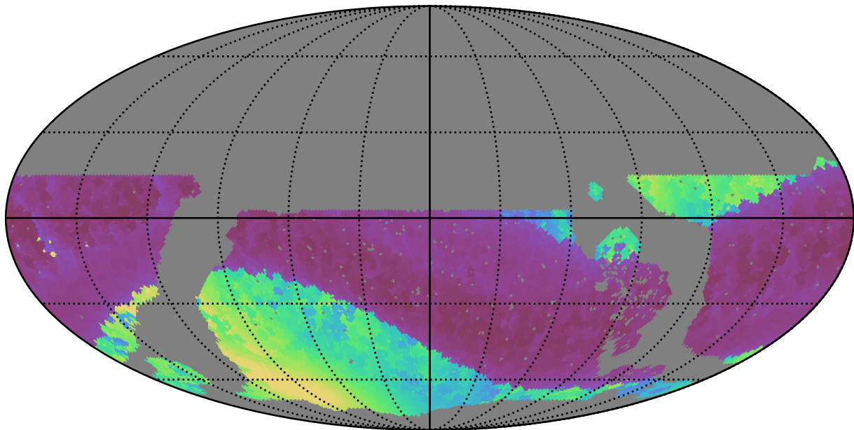
noroll_mjdp120_v3.4_10yrs WFD all bands: Min solarElong
