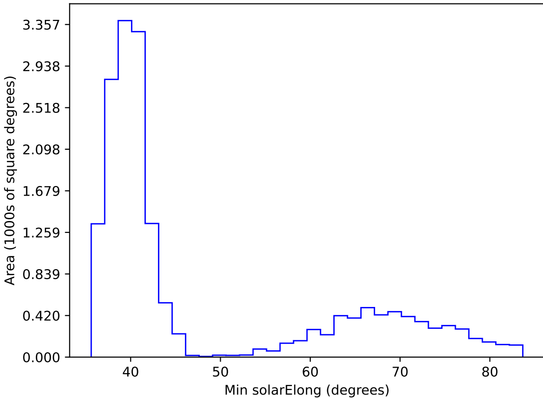
noroll_mjdp120_v3.4_10yrs WFD all bands: Min solarElong
