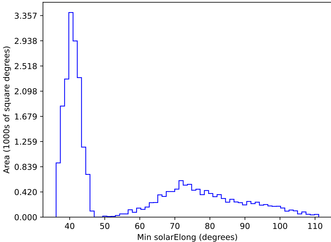
noroll_mjdp120_v3.4_10yrs All sky z band: Min solarElong
