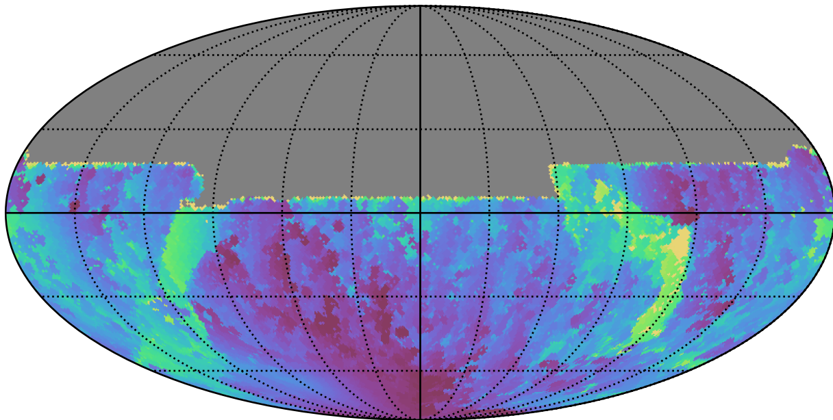
noroll_mjdp120_v3.4_10yrs All sky u band: Min solarElong
