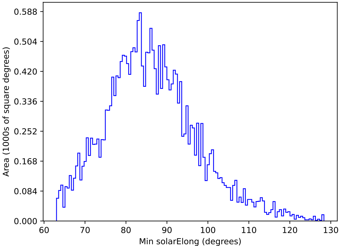
noroll_mjdp120_v3.4_10yrs All sky u band: Min solarElong
