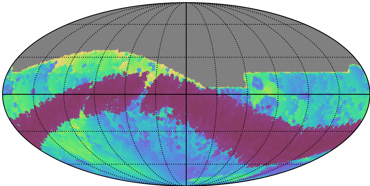
noroll_mjdp120_v3.4_10yrs All sky r band: Min solarElong
