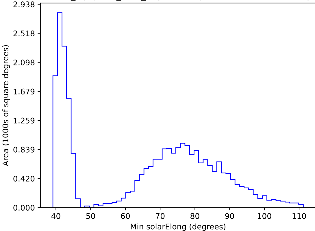
noroll_mjdp120_v3.4_10yrs All sky r band: Min solarElong
