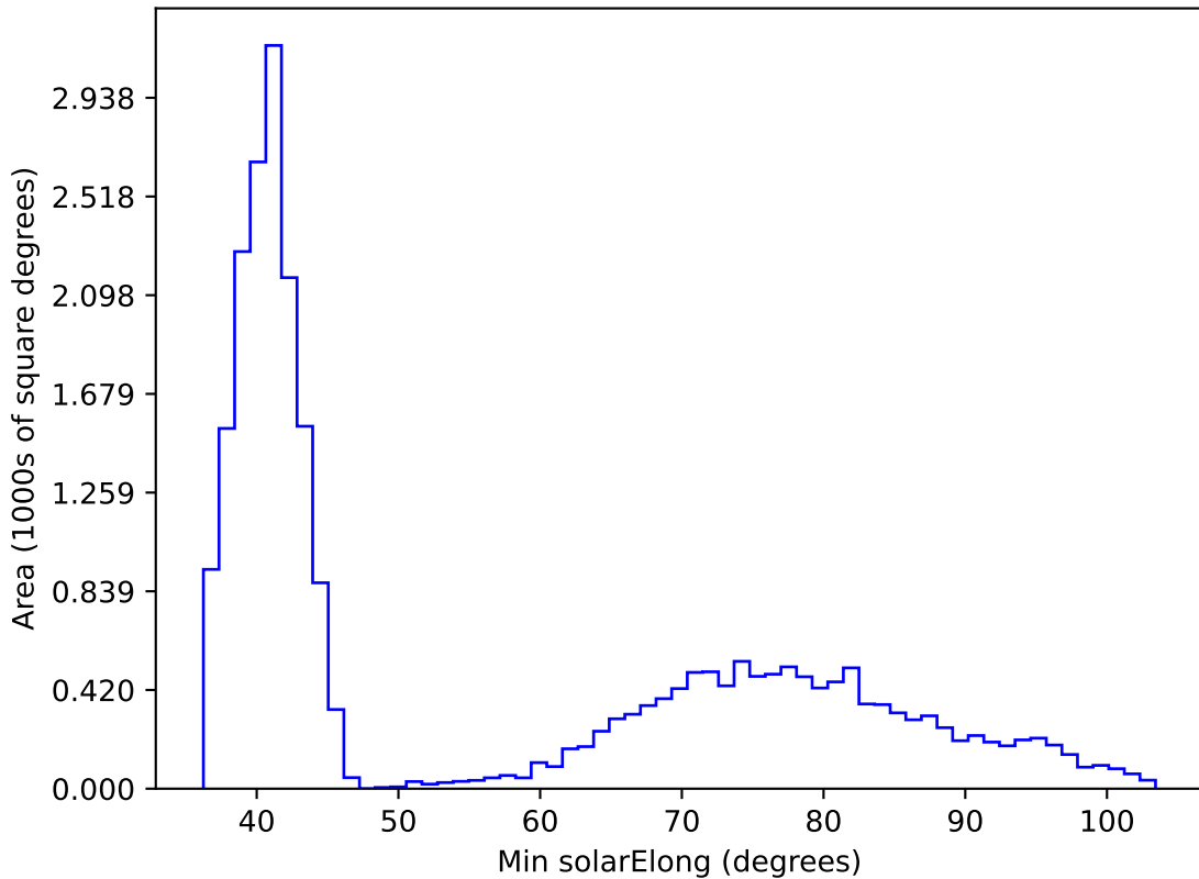
noroll_mjdp120_v3.4_10yrs All sky i band: Min solarElong
