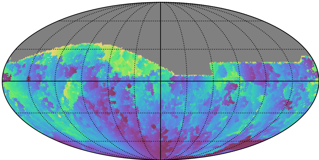
noroll_mjdp120_v3.4_10yrs All sky g band: Min solarElong
