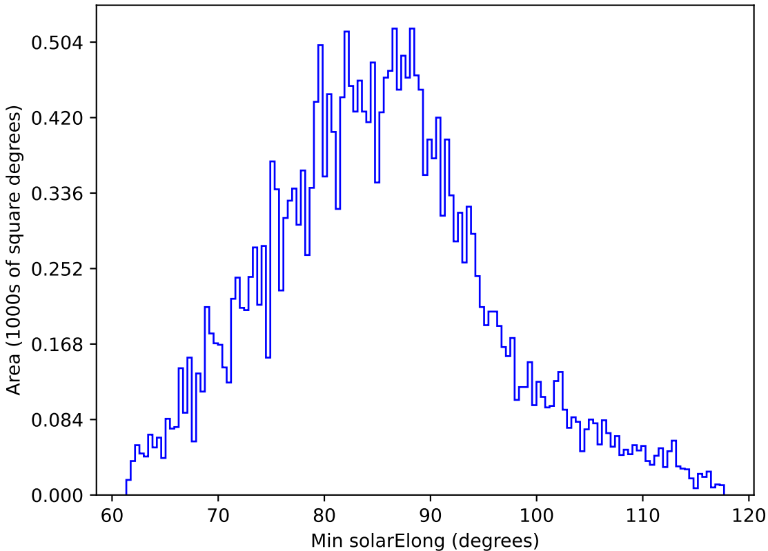
noroll_mjdp120_v3.4_10yrs All sky g band: Min solarElong
