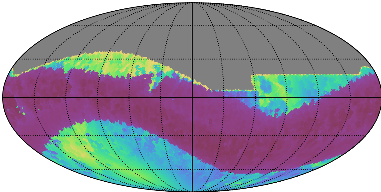
noroll_mjdp120_v3.4_10yrs All sky all bands: Min solarElong
