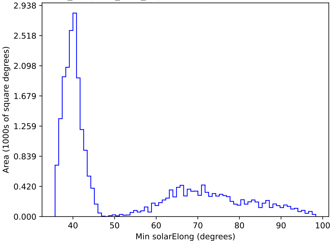
noroll_mjdp120_v3.4_10yrs All sky all bands: Min solarElong
