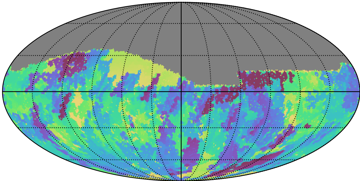
noroll_mjdp120_v3.4_10yrs Yr 1 r band: Min skyBrightness
