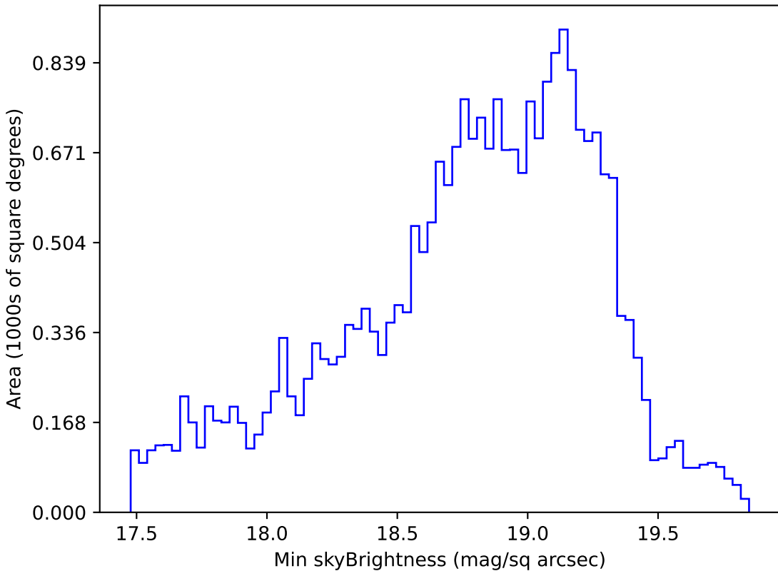
noroll_mjdp120_v3.4_10yrs Yr 1 i band: Min skyBrightness
